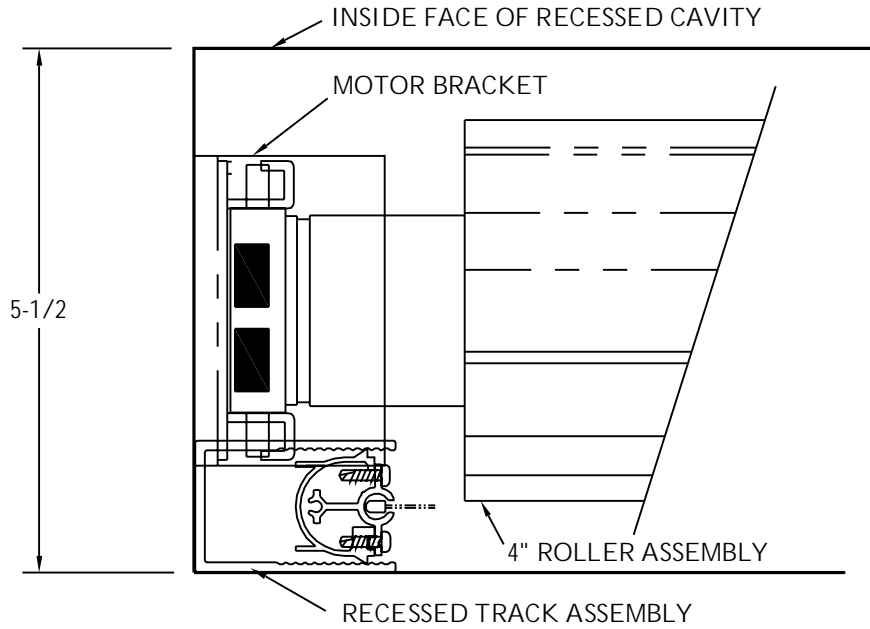
MINIMUM RECESSED CAVITY WITH A 4" ROLLER
