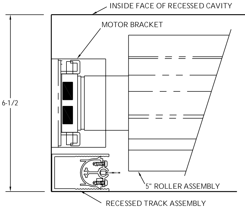
MINIMUM RECESSED CAVITY WITH A 5" ROLLER
