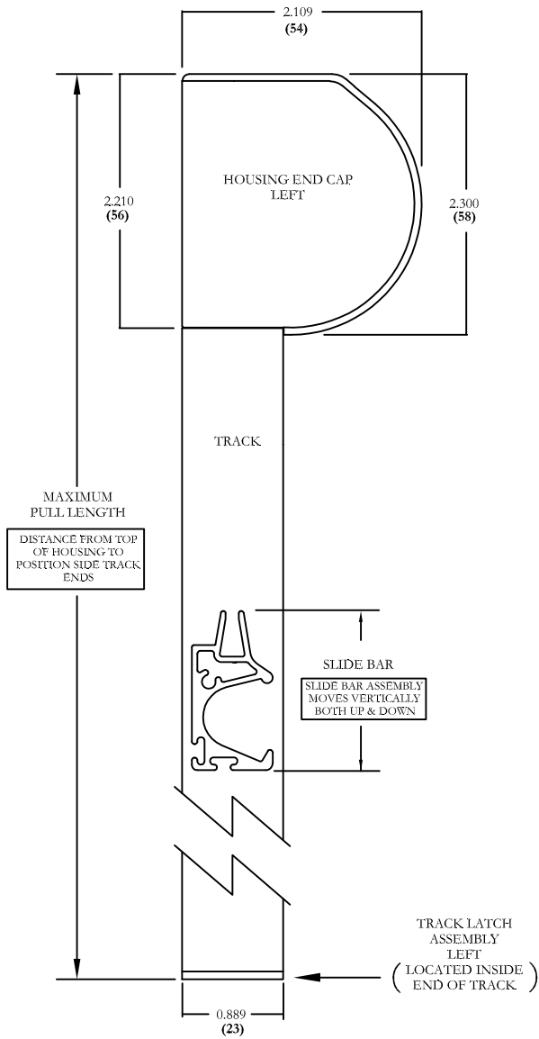
SERENE WINDOW SCREEN ASSEMBLY LEFT SIDE VIEW
